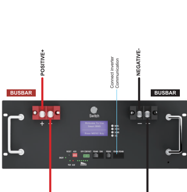
Schematic Diagram of Connection and Use Of Single Battery
