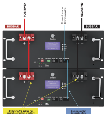
Schematic Diagram of Connection and Use Of Two Batteries
